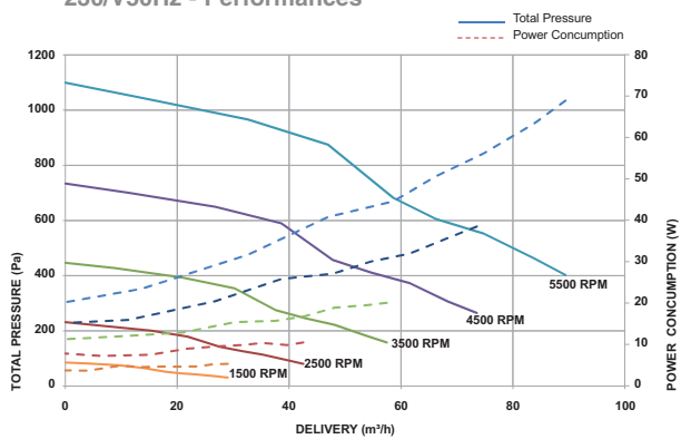
230V/50Hz - Performances
