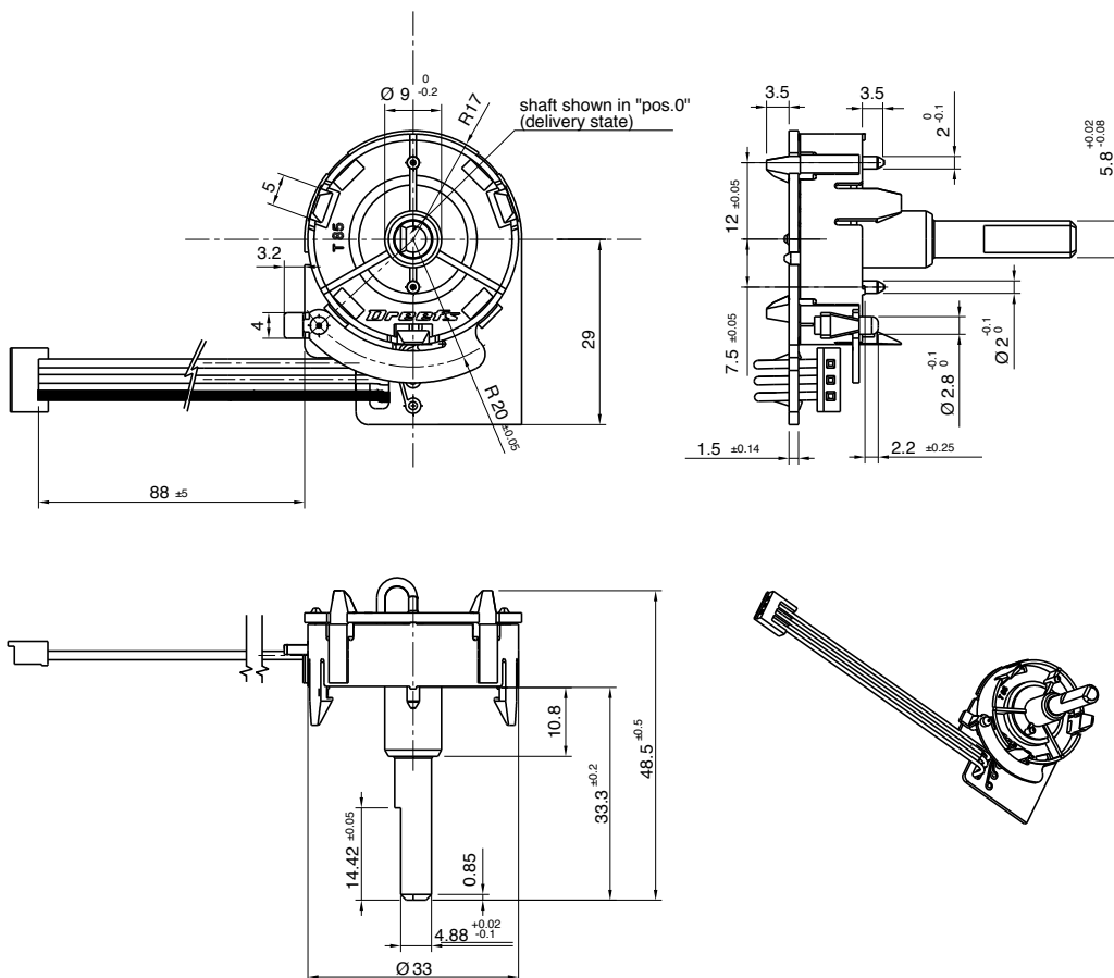
MF encoder, standard body version with snap in fixing type or self snapping fixing type.
